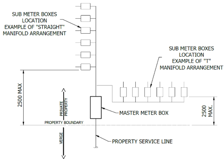
Fig. 8.6.1 Typical Sub-Meter "T" and "Straight" arrangements
