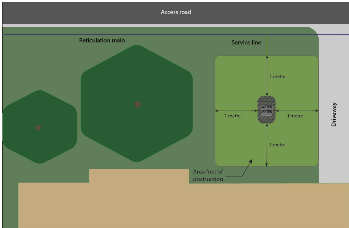
Fig. 7.4.1A Minimum Clearances for DN20 Water Meters in Meter Boxes
