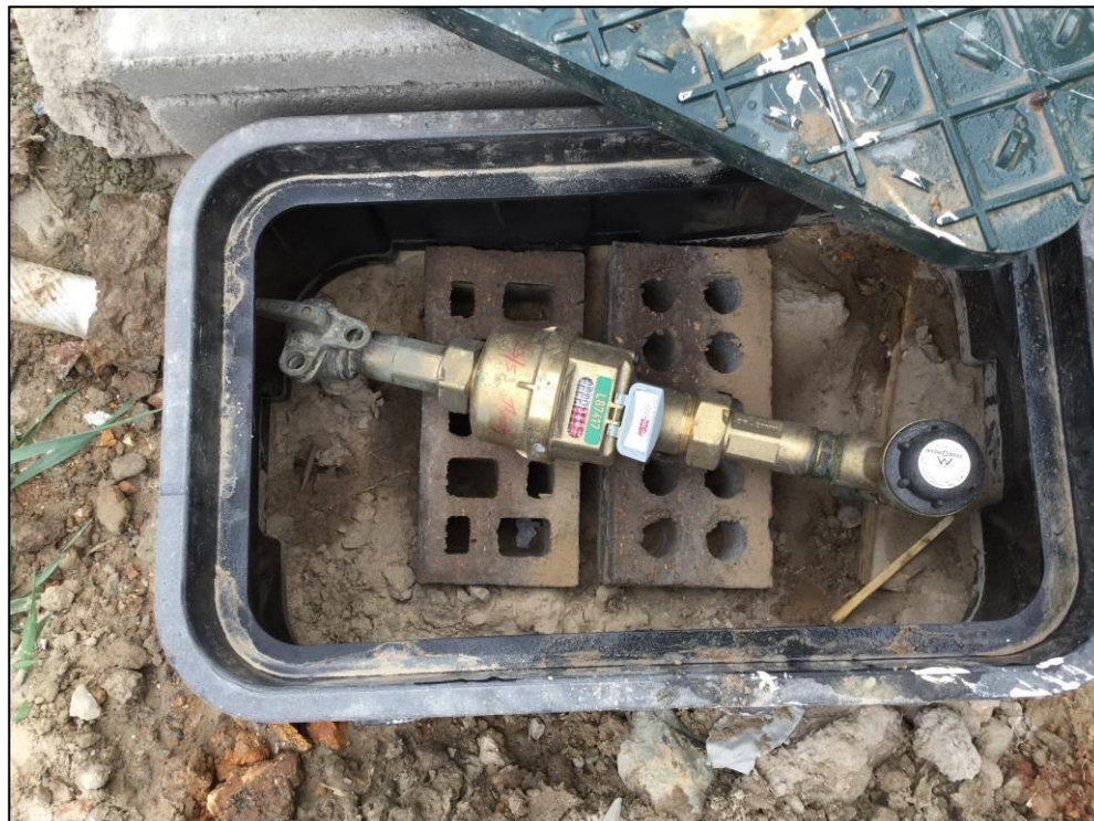
Fig. 10.2 Failed DN20 Water Meter Installation (Not centred; reduced valve clearance; PRV in box)
