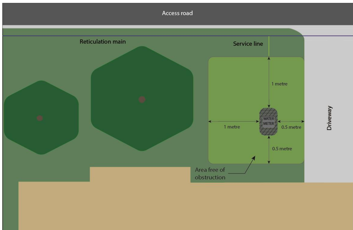
Fig. 7.4.1B Minimum Clearances for DN20 Water Meters in Meter Boxes – Special Approval
