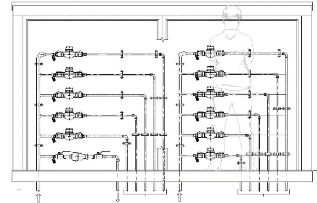
Fig. 8.6.2 Typical Sub-Meter Cabinet assembly – Elevation
