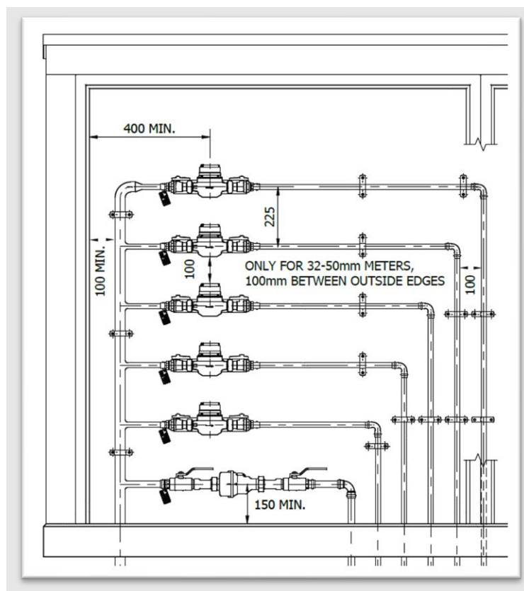
Figure 5.6.7 The clearances in the meter cabinet
