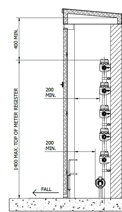
Figure 5.6.8 The required clearances in the meter cabinet inside view
