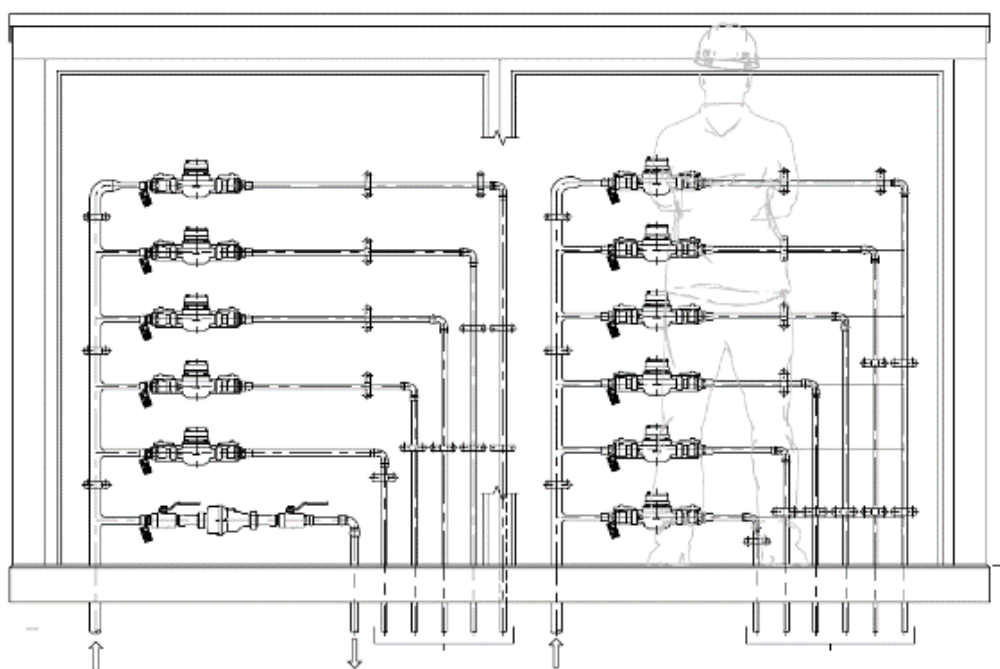
Figure 5.6.4 Typical Sub-Meter Cabinet assembly – Elevation
