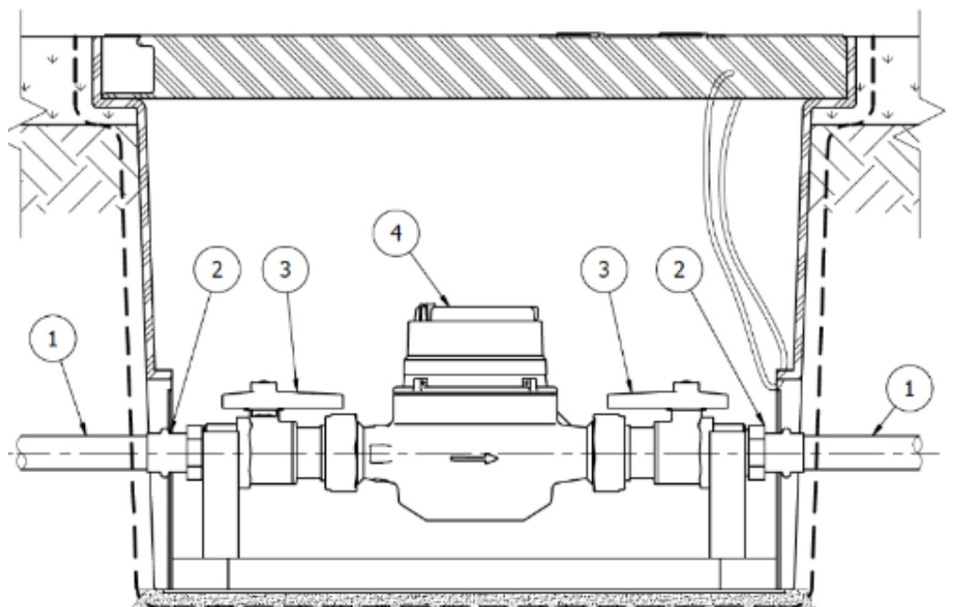
Figure 5.5.2 Approved Water Sub-Meter DN20 – Inground pit installation
