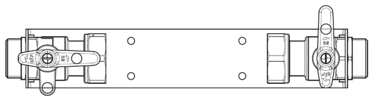
Figure 5.6.9 Typical cabinet mount bracket with ball valves
