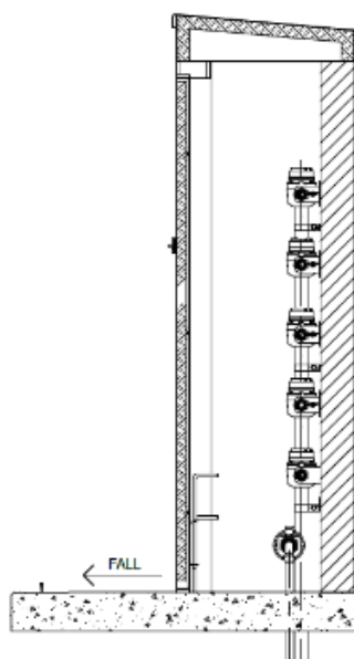
Figure 5.6.4 Typical Sub-Meter Cabinet assembly – Elevation
