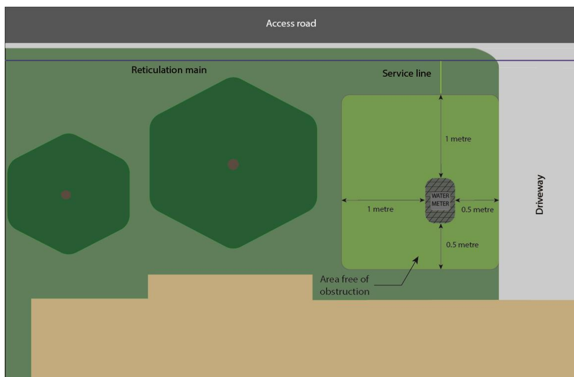
Figure 4.4.2 Minimum Clearances for DN20 Water Meters in Meter Boxes – Special Approval
