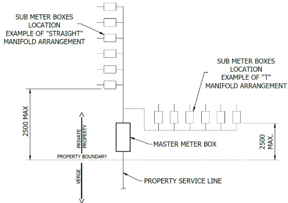
Figure 5.6.1 Typical Sub-Meter “T” and “Straight” arrangements
