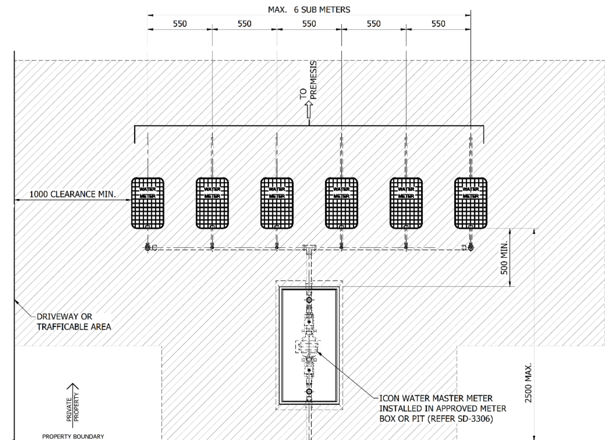
Figure 5.6.2 Typical Sub-Meter box assemblies – plan view
