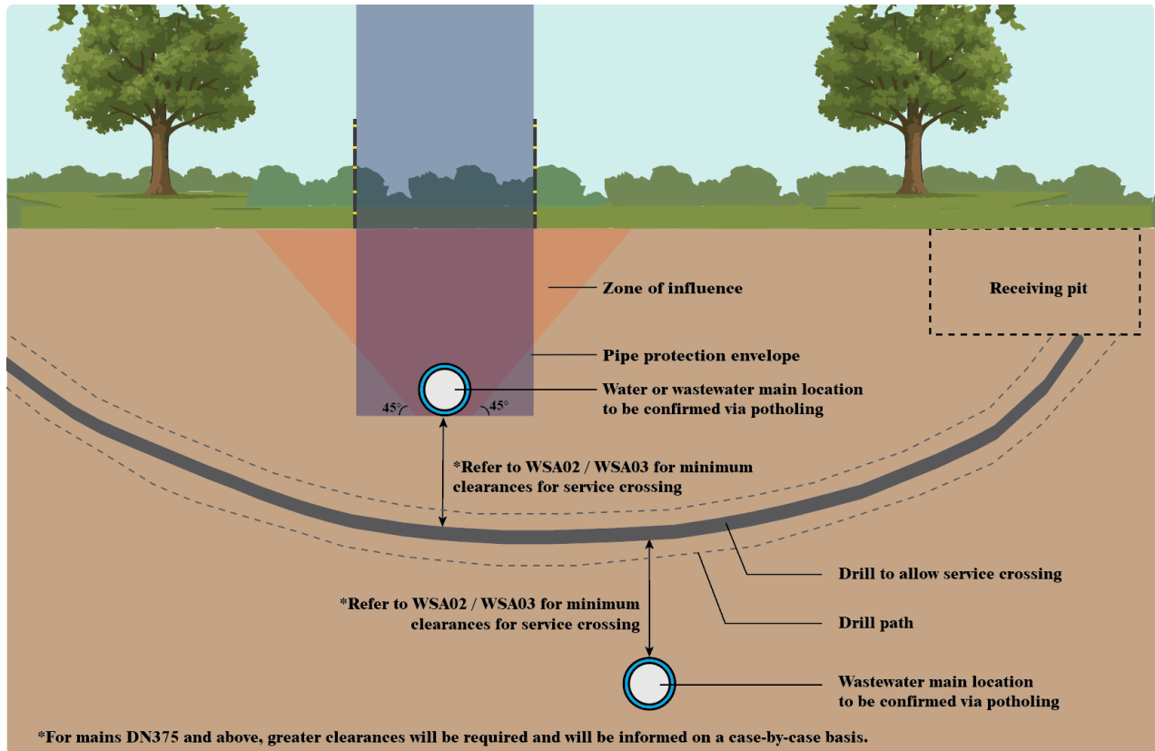
Figure 5.6.1 Requirements for horizontal directional drilling
