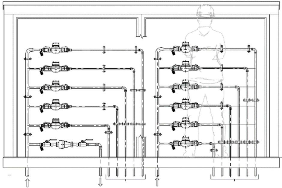
Figure 5.5-4 Typical sub-meter Cabinet assembly – Elevation
