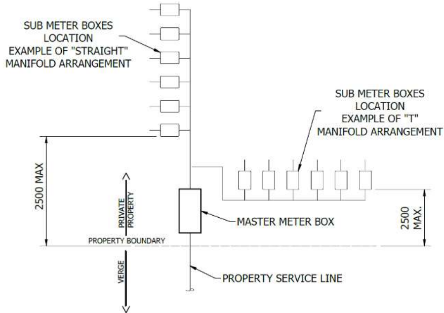
Figure 5.5-1 Typical sub-meter “T” and “Straight” arrangements
