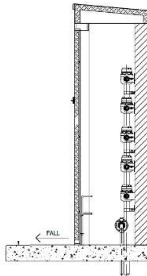
Figure 5.5-4 Typical sub-meter Cabinet assembly – Elevation
