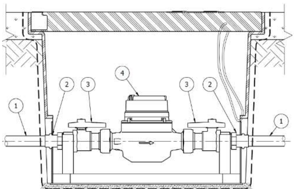
Figure 5.4-2 Approved water sub-meter DN20 – Inground box installation
