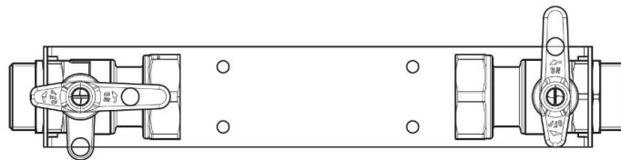
Figure 5.5-7 Typical meter bracket with ball valves
