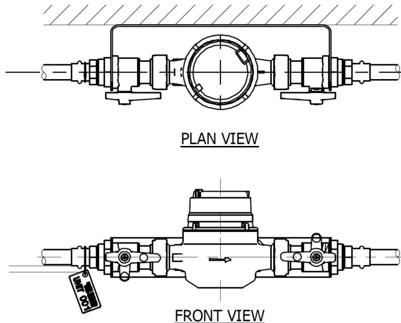
Figure 5.4-3 Approved water sub-meter DN20 – Above ground enclosure installation with Stainless Steel or PE bracket
