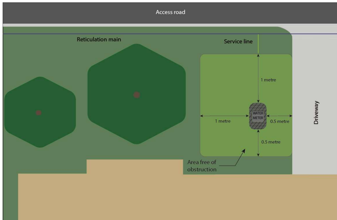
Figure 4.4-2 Minimum Clearances for DN20 Water Meters in Meter Boxes – Special Approval
