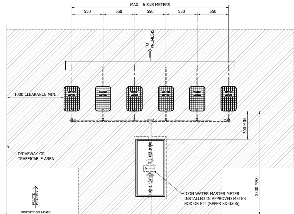
Figure 5.5-2 Typical sub-meter box assemblies – plan view
