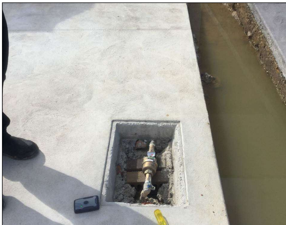
Figure Appendix A4 Failed DN20 Water Meter Installation (water meter in driveway and meter too high)
