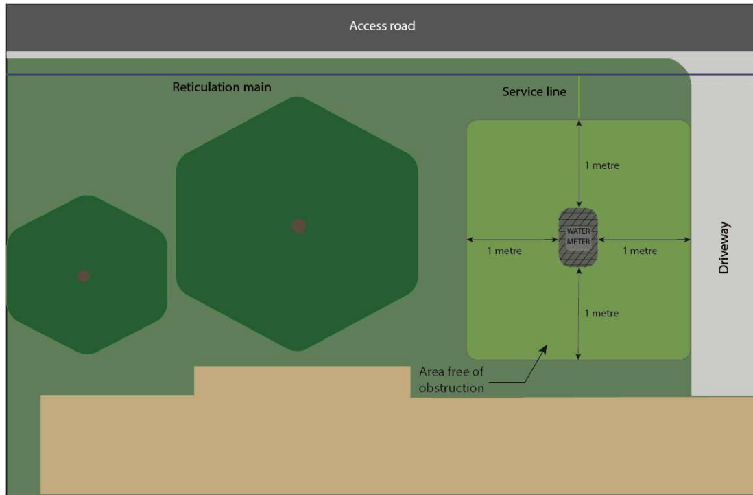
Figure 4.4-1 Minimum Clearances for DN20 Water Meters in Meter Boxes
